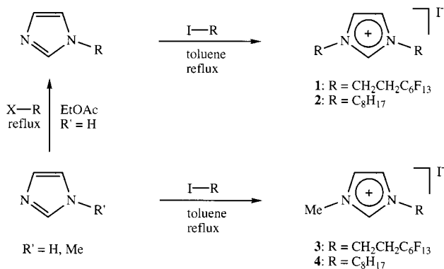
Scheme 1. Preparation of imidazolium salts.
