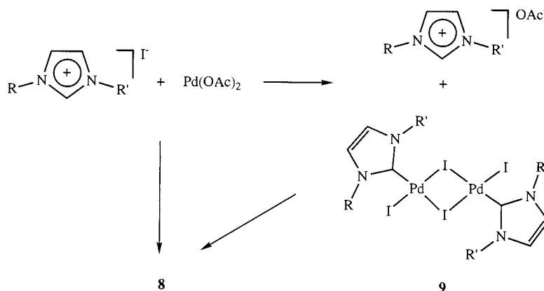
Scheme 3. Formation of 8 via binuclear complex 9 ( \text{R} = \text{C}_8\text{H}_{17} , \text{R}' = \text{Me} ).
